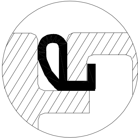
Detail "A" Neoprene "P" Bulb Gasket
