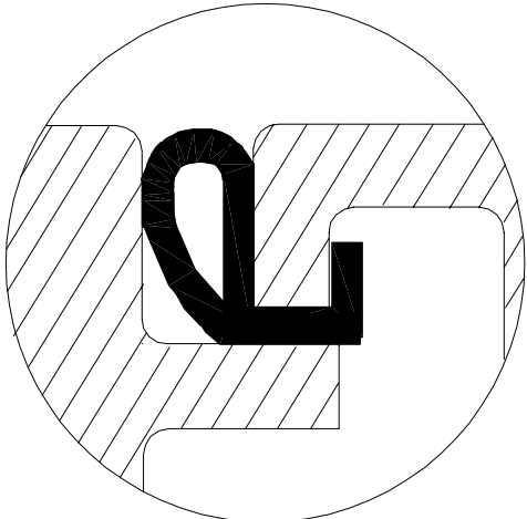
Detail "A" Neoprene "P" Bulk Gasket
