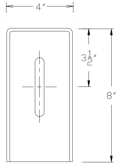
Lower Bracket
