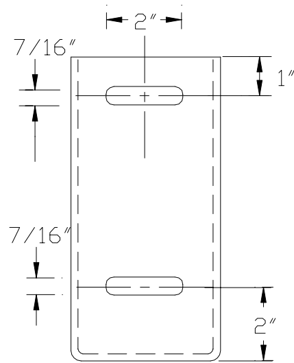
Upper Bracket
