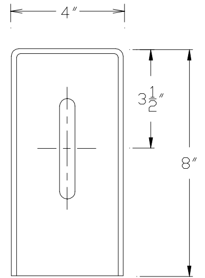
Lower Bracket
