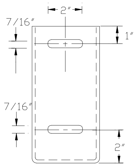
Upper Bracket
